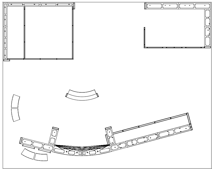
Plan View 50' 30'
